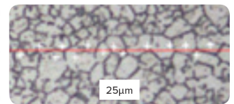
Datum PhD Microstructure Grain Size: 7-11µm
